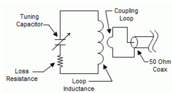
Equivalent Circuit [3]
